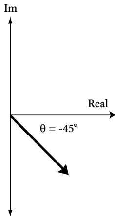
Figure 3. Phasor plot for a non-ideal capacitor.
